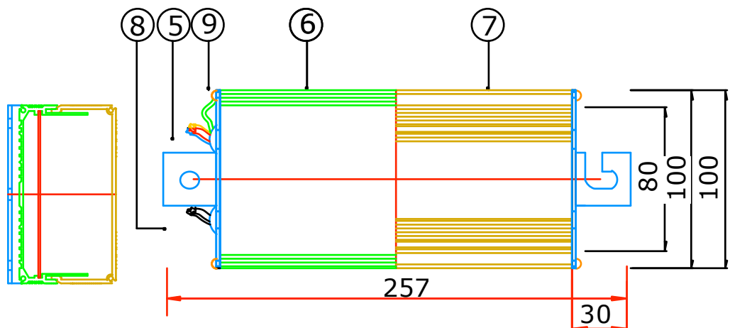
TOP VIEW OF BALLAST
