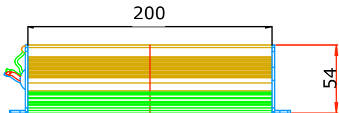
FRONT VIEW OF BALLAST
